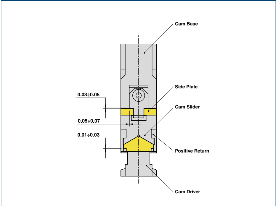
SLIDER STRUCTURE, POSITIVE RETURN STRUCTURE AND CLEARANCES
