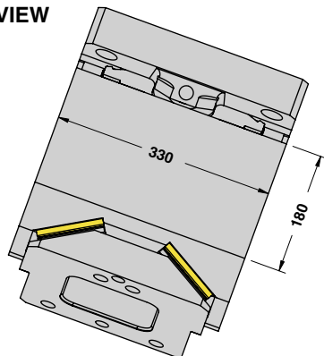
CAM DIAGRAM
