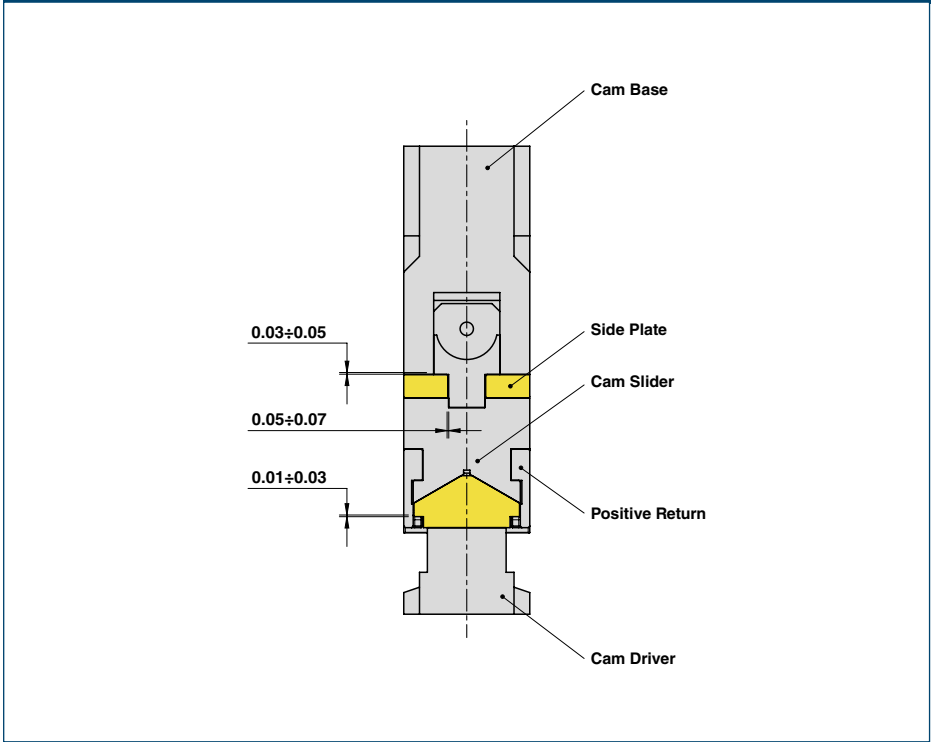
SLIDER STRUCTURE, POSITIVE RETURN STRUCTURE AND CLEARANCES
